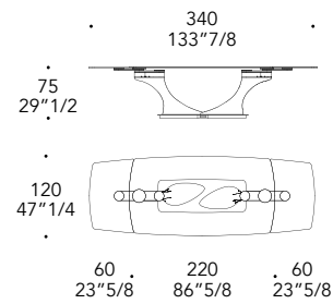
EXTENDABLE Square-round 220-340
