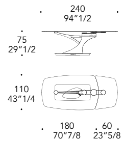
EXTENDABLE Square-round 180-240
