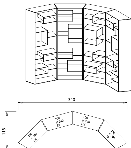
Comp. 3 340 x 118 x h 240 2 x 100 h 240 dx + 2 x 100 h 240 sx
